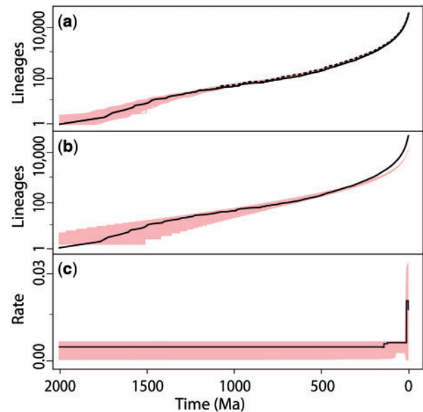
FIG. 4. (1 column) Patterns of lineage diversification. (a) Cumulative lineages-through-time (LTT) curve for eukaryotes (50,455 sp.), in black, showing the number of lineages through time (unsmoothed, dashed; smoothed, solid) and variance (red, 500 replicates). (b) Same LTT curve (black line), but compared with a simulated constant-expansion LTT curve ( \lambda (speciation rate) = 0.073 and \mu (extinction rate) = 0.070) shown as \pm 99% confidence intervals (red). (c) Diversification rate plot of same data showing only significant changes in rate as determined in maximum-likelihood tests; variance (red, 500 replicates) shown as \pm 99% intervals.
